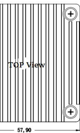
Standard+Heatsink 61*57.9*27.7mm
